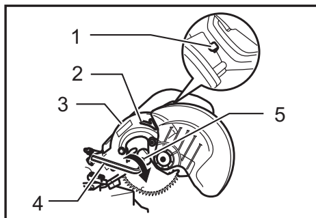
► 1. Shaft lock 2. Arrow 3. Blade case 4. Hex wrench 5. Hex socket bolt
