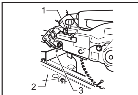
► 1. Adjusting bolt 2. Turn base 3. Guide fence
