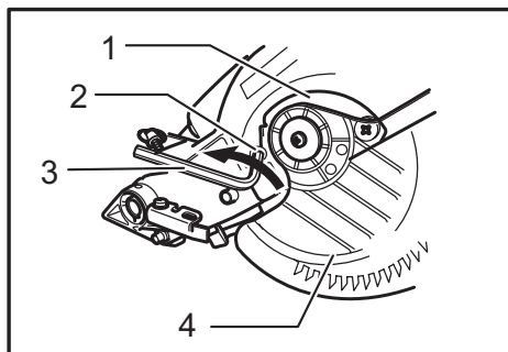
► 1. Center cover 2. Hex socket bolt 3. Hex wrench 4. Safety cover
